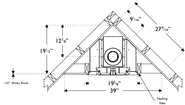
MQ19ZDV Corner Framing Dimensions (inches)
